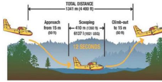
Source: United States Department of Agriculture Amphibious Water Scooper Aircraft Operations Plan 2016.
